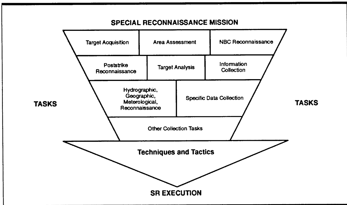
Figure 1-2. SR tasks.
